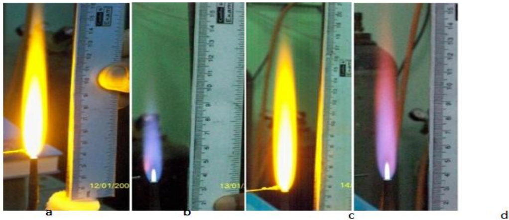
Fig. 13: Photographs of the flames with BMCG and LPG at flow rate 0.1 SLM a) LPG with sodium seeding b) LPG without sodium seeding c)BMCG with sodium seeding d) BMCG without sodium seeding
