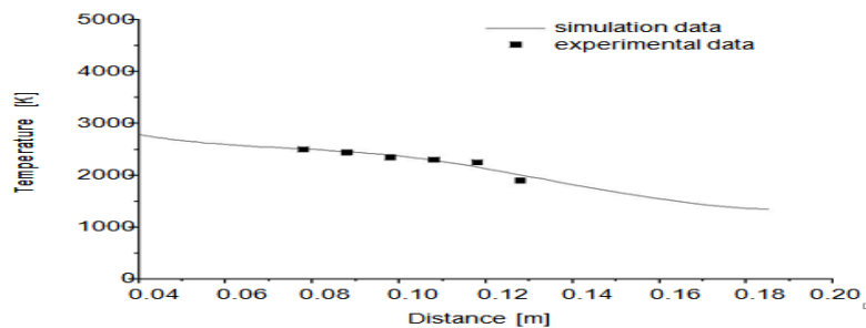
Fig 9 : Comparison of computed and experimental axial values of temperature for 0.1 SLPM
