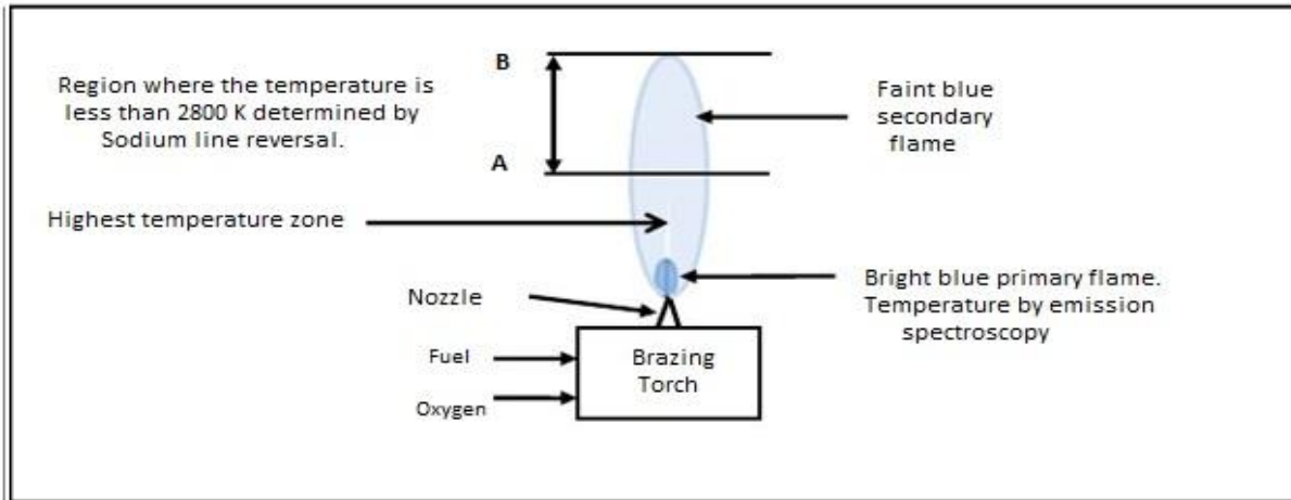
Fig.1: Flame resulting from fuel burned in a brazing torch.
