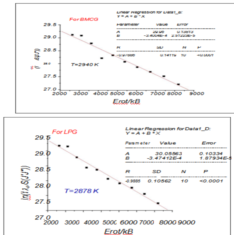
Fig. 5: Typical Boltzmann plot for CH* rotational spectrum for BMCG for LPG flames. (Temperatures: 2940 K and 2878 K respectively)
