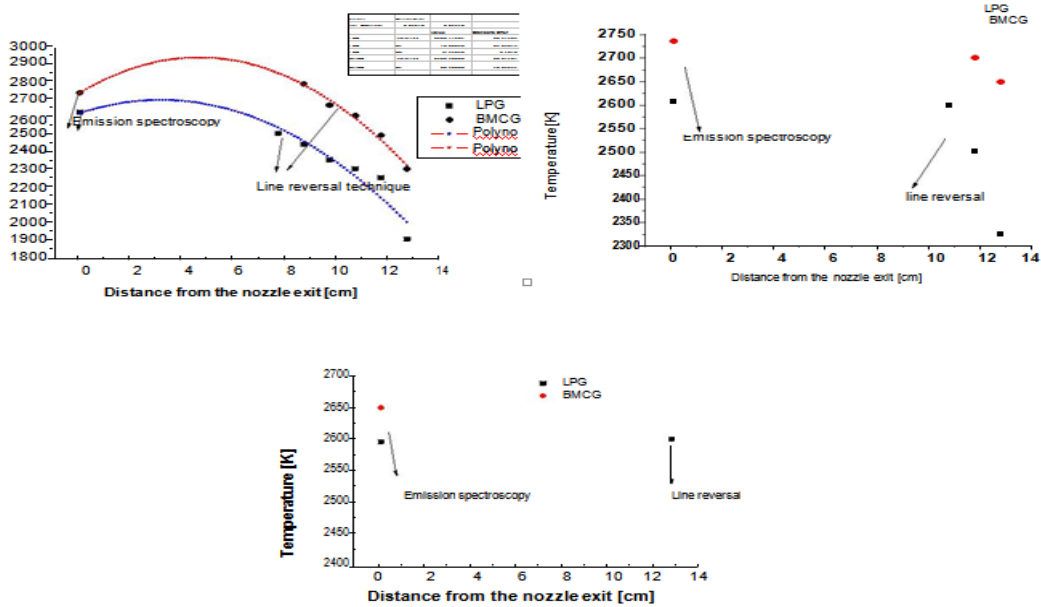
Fig. 12: Temperature profile for LPG and BMCG flames at fuel flow rate of a) 0.1 SLM b) 0.14 SLM c) 0.18 SLM
