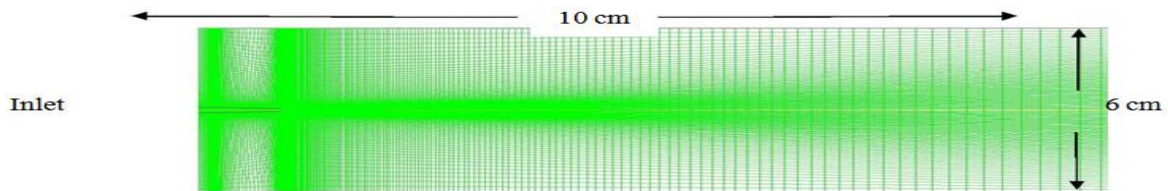
Fig 8 : Computational domain
