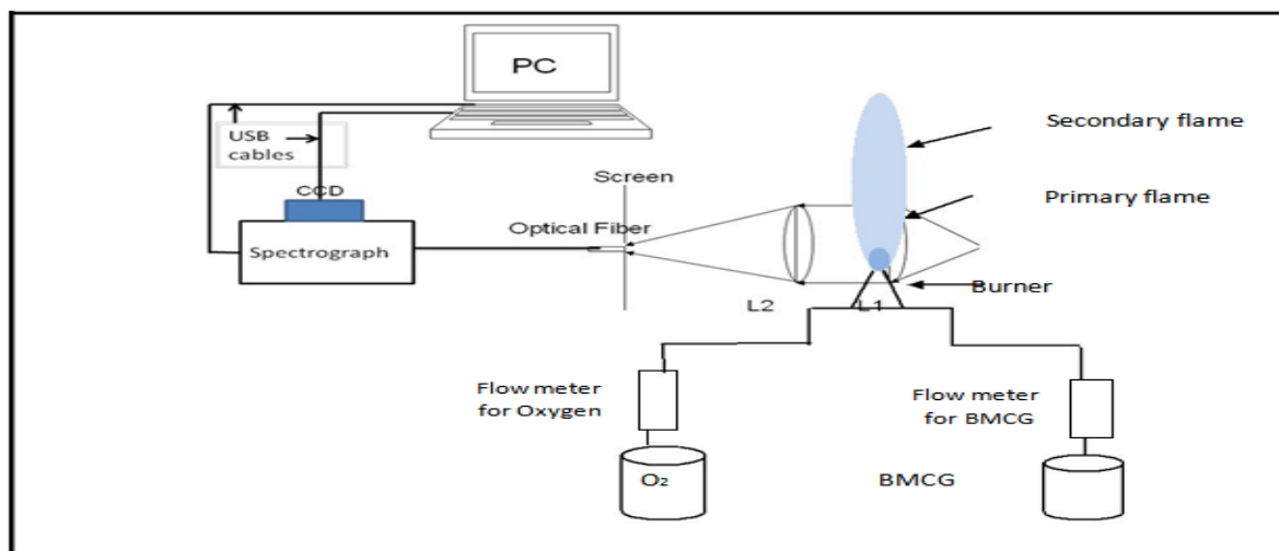
Fig. 3: Experimental setup for spectroscopic determination of primary flame temperature.
