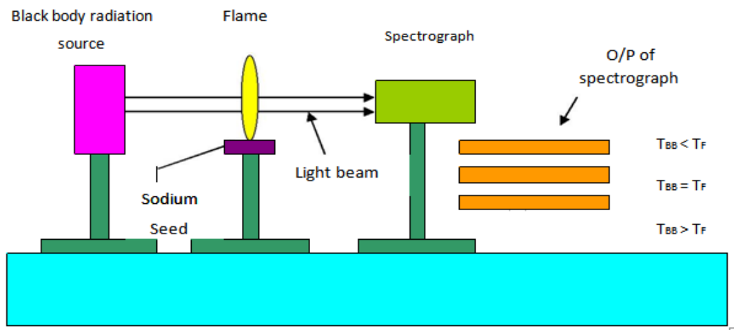
Fig. 2: Line reversal technique: schematic of experimental arrangement
