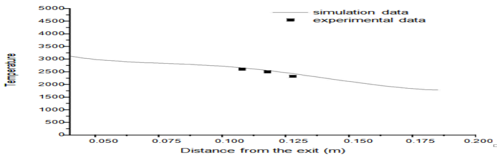
Fig10 : Comparison of computed and experimental axial values of temperature for 0.14 SLPM
