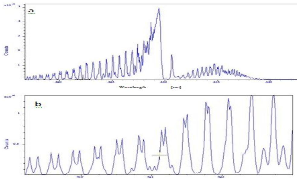
Fig. 4: a) Typical vibration-rotation band around 431.5 nm b) Expanded view of rotation spectrum
