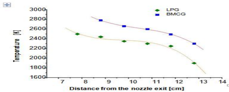
Fig.11: Axial temperature profile of flame by LPG and BMCG at fuel flow rate of 0.1 SLM and Oxygen just above stoichiometry (Just Oxidizing flame).
